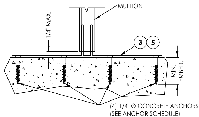
4 4 ANCHOR BRACKET DETAIL Anchor Direct to Masonry
