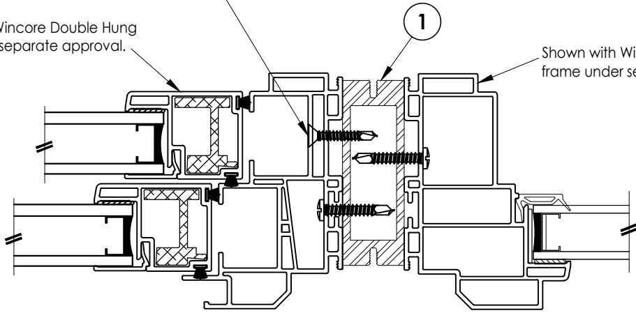
1 2 FRAME TO MULLION CONNECTION
