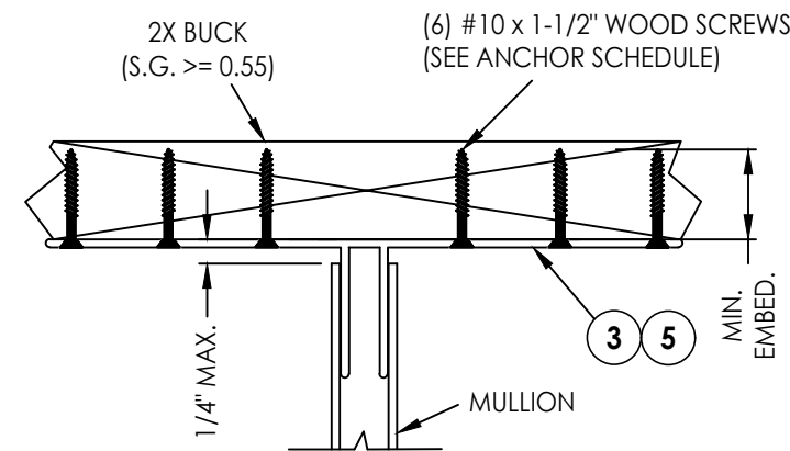
1 4 ANCHOR BRACKET DETAIL Anchor to 2x Buck
