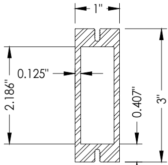
1 TMP-2603 MULLION 6063-T6 ALUM.
